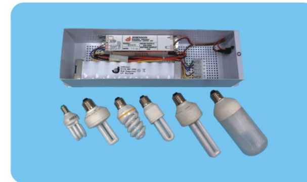
JF23SLN2, Emergency SL conversion kit. It can be suitable for different energy saving lamps.
