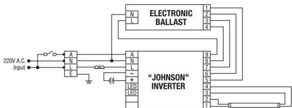
6V, 12V Electronic Ballast (電子牛)
