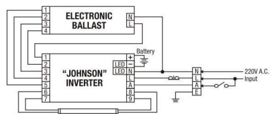
18V Electronic Ballast (電子牛)
