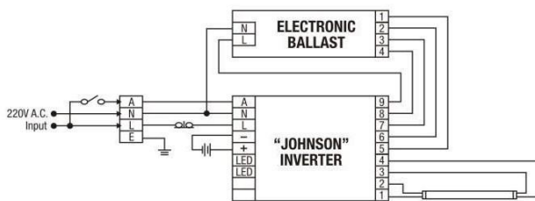
9.6V, 12V Electronic Ballast (電子牛)
