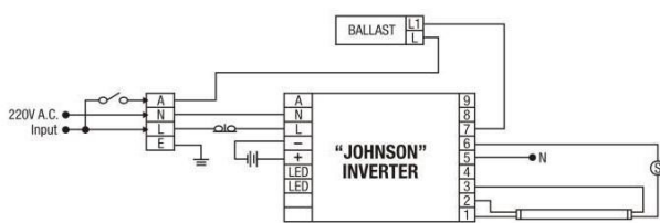
9.6V, 12V Conventional Ballast (鎮流器)
